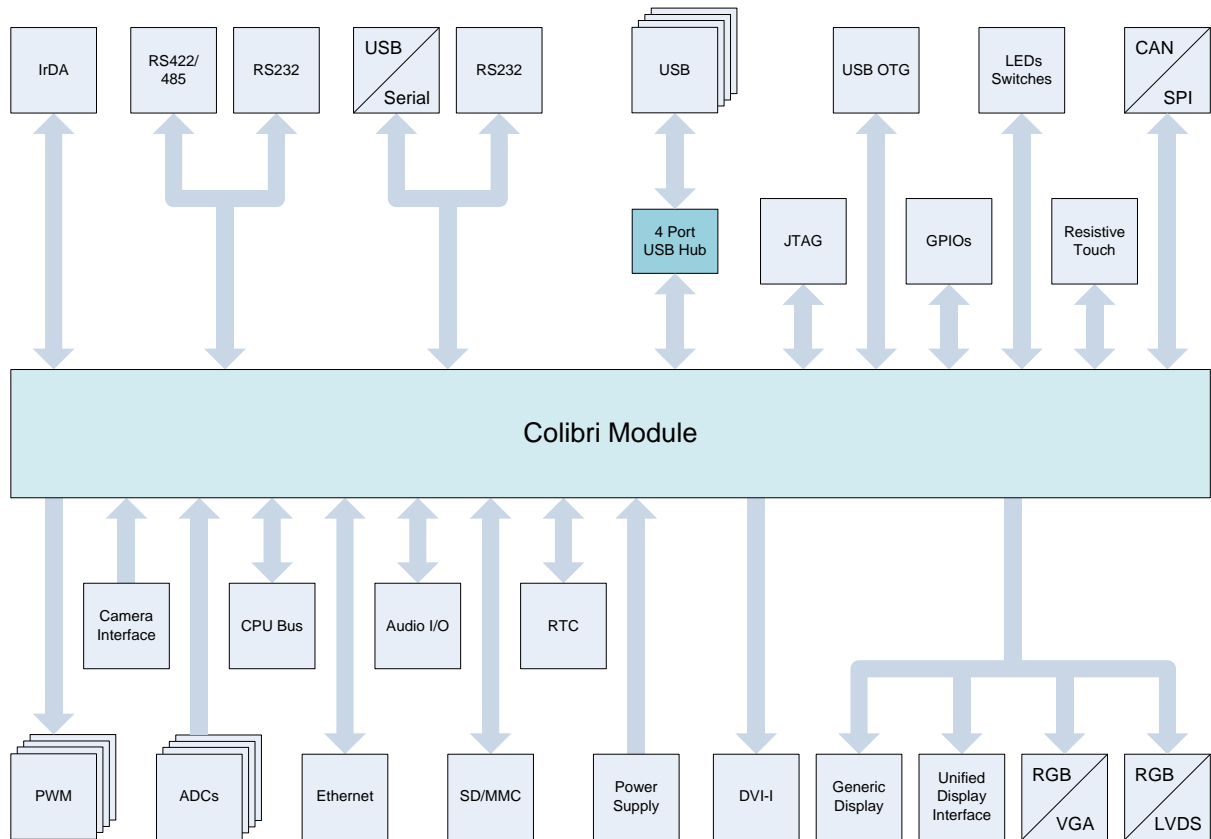
Fig.1 Colibri Evaluation Board Hardware Architecture
